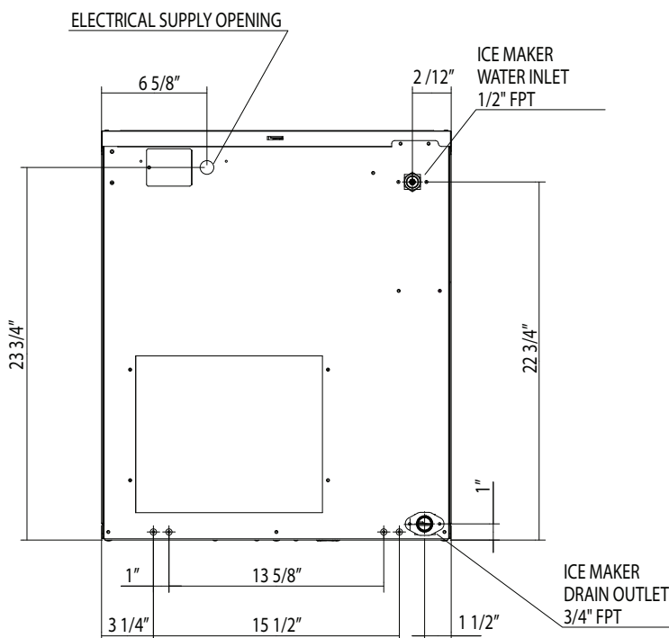
REAR VIEW
