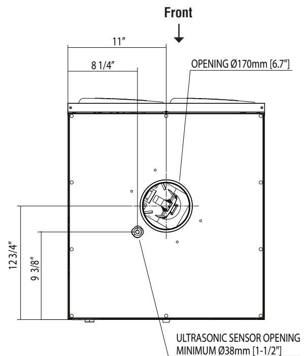
BOTTOM VIEW
