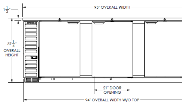
Elevation View
