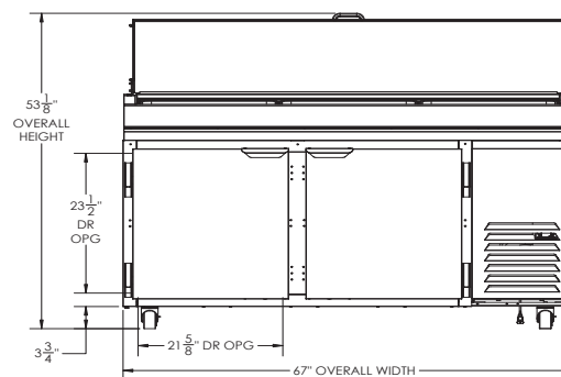
ELEVATION VIEW
