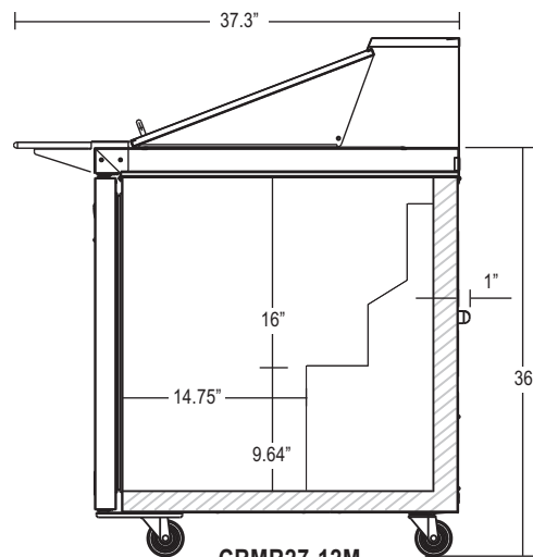
CRMR27-12M SIDE (Cross Section)
