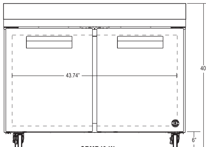
CRMR48-W FRONT
