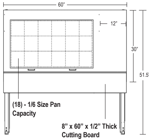
CRMR60-18M PLAN VIEW
