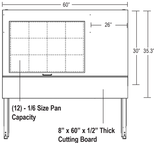
CRMR60-12M PLAN VIEW
