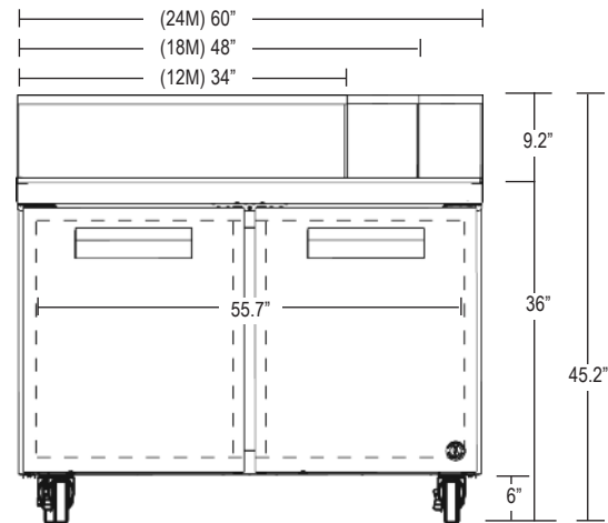
CRMR60 (-12M/-18M/-24M) FRONT
