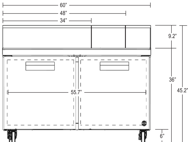
CRMR60 (-8/-12/-16) FRONT
