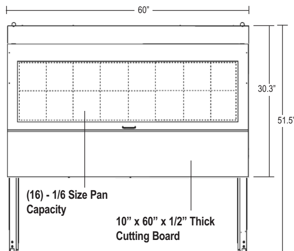
CRMR60-16 PLAN VIEW
