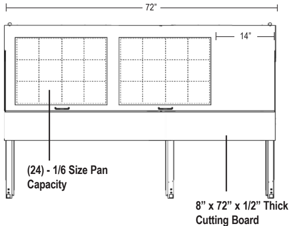
CRMR72-24M PLAN VIEW
