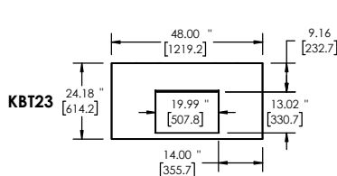
PLAN / TOP VIEW
