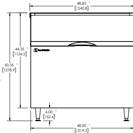
ELEVATION / FRONT VIEW
