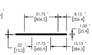
ELEVATION / FRONT VIEW
