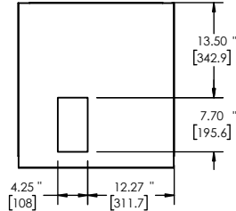
PLAN / TOP VIEW
