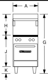
Dimensions - in(mm)
