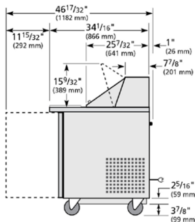
RIGHT VIEW
