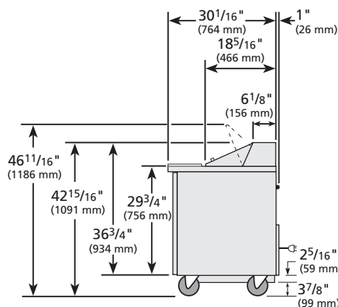
RIGHT VIEW
