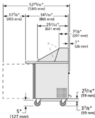
RIGHT VIEW
