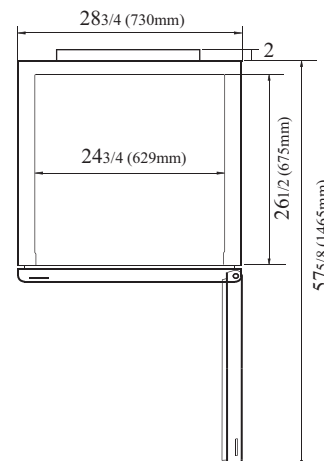
PLAN VIEW
