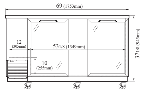
TBB-3SG FRONT VIEW
