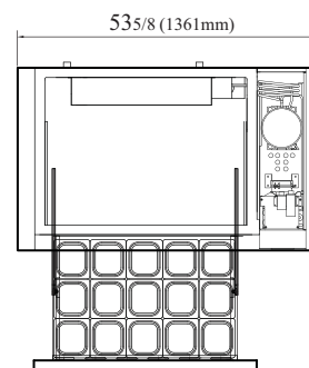
EXTENDED TOP PLAN VIEW
