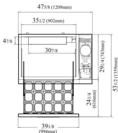
PLAN VIEW
