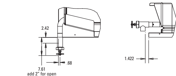
2" Draw-off valve – left side 90° front (BPDOV-3)
