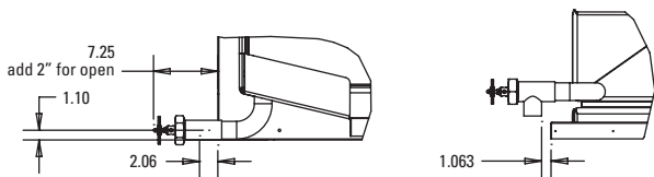
2" Draw-off valve – left front 90° left (BPDOV-2)
